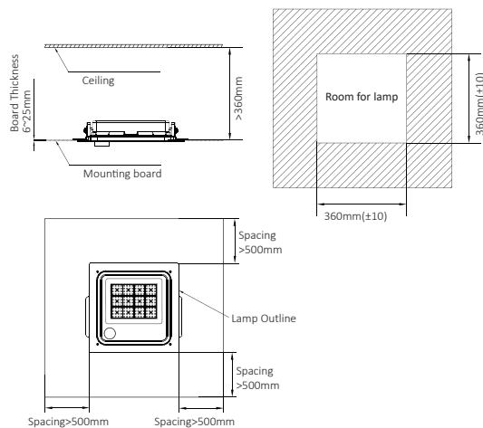
Recessed Mounting
